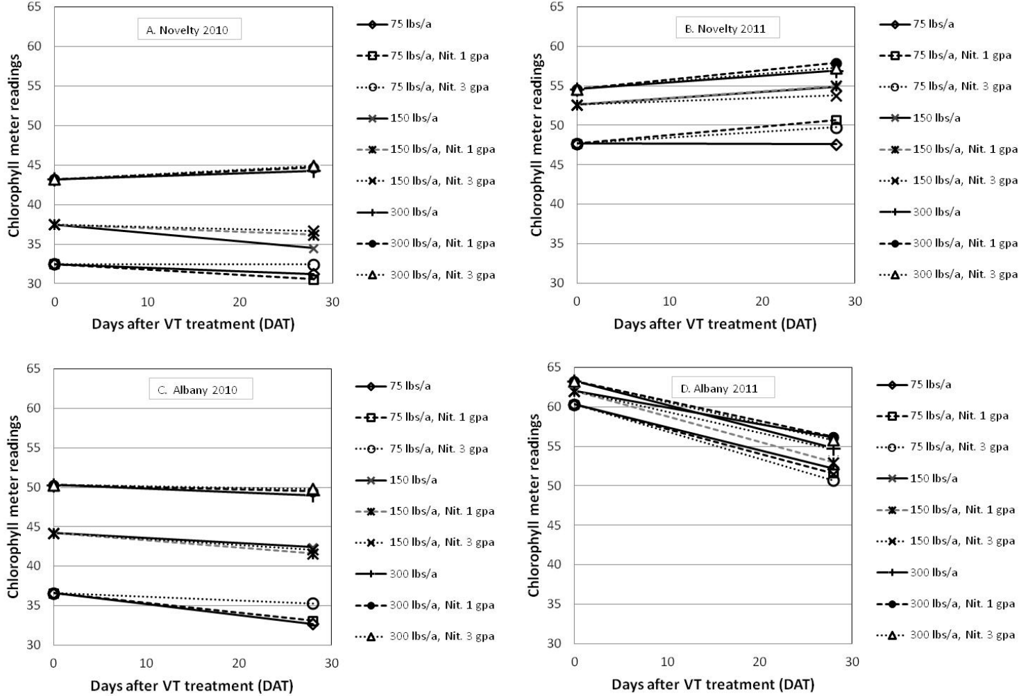
Figure 1. Chlorophyll meter readings at the time of application (VT) and 28 days after treatment (DAT) soil applied N treatments (75, 150, or 300 lbs N/acre) and Nitamin (Nit.) rates ( 0, 1 or 3 gallons per acre = gpa) at Novelty (2010 and 2011) and Albany (2010 and 2011). Data were combined over Headline treatments. LSD ( P=0.1 ) is 1.
